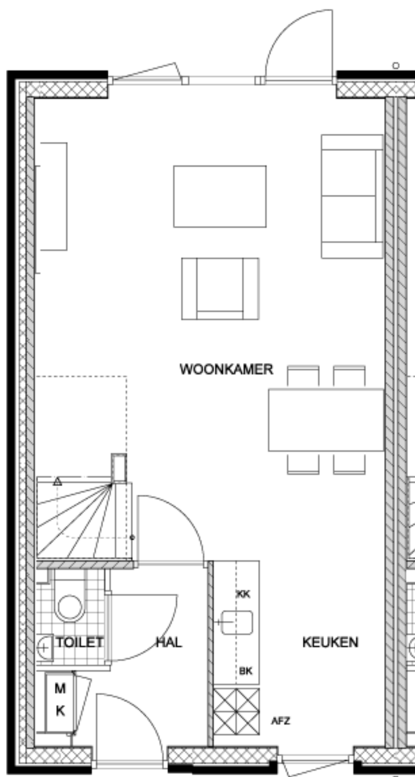
BEGANE GROND 1: 50
